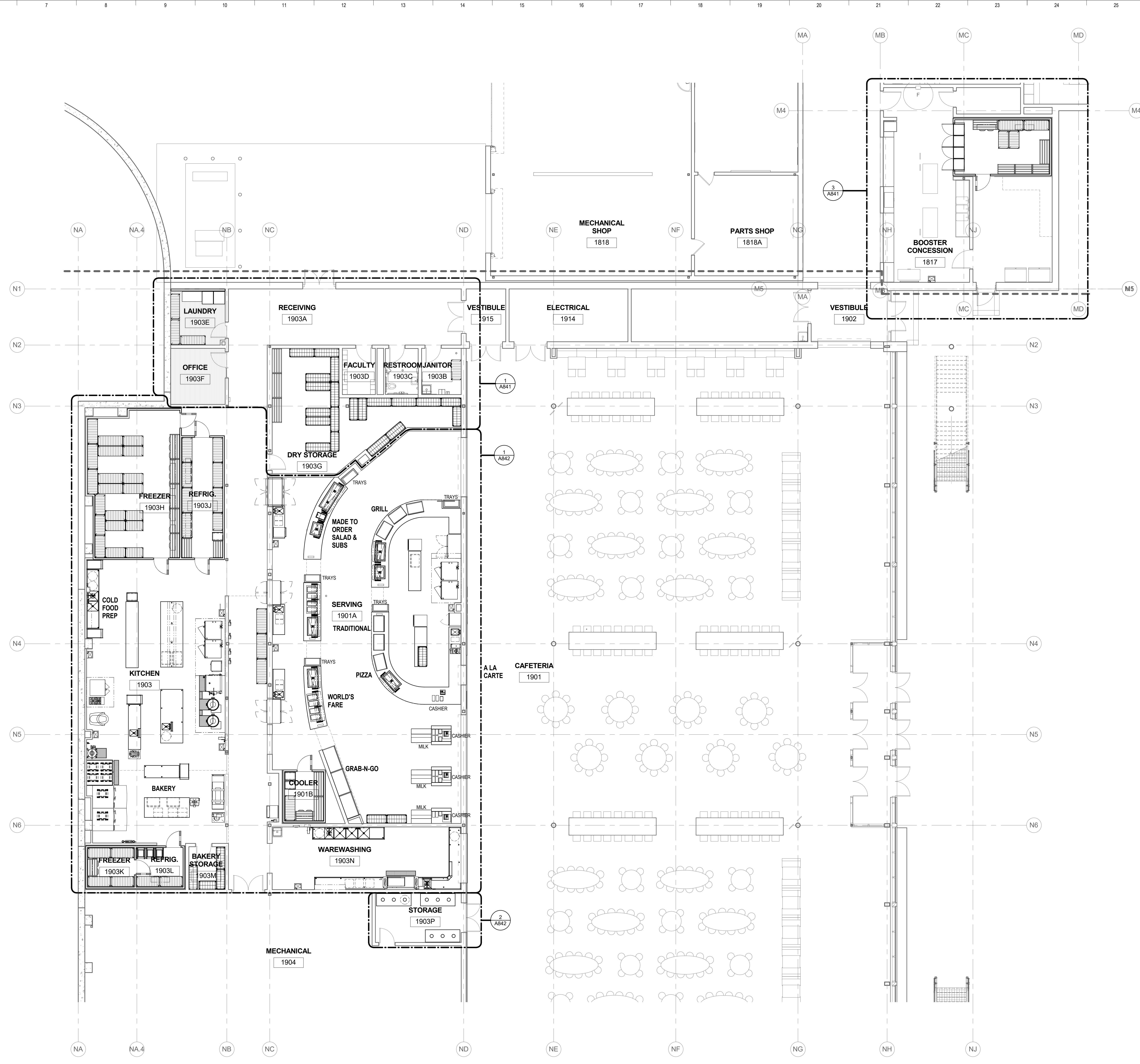
1 FOODSERVICE EQUIPMENT OVERALL PLAN 1/8" = 1'-0"
