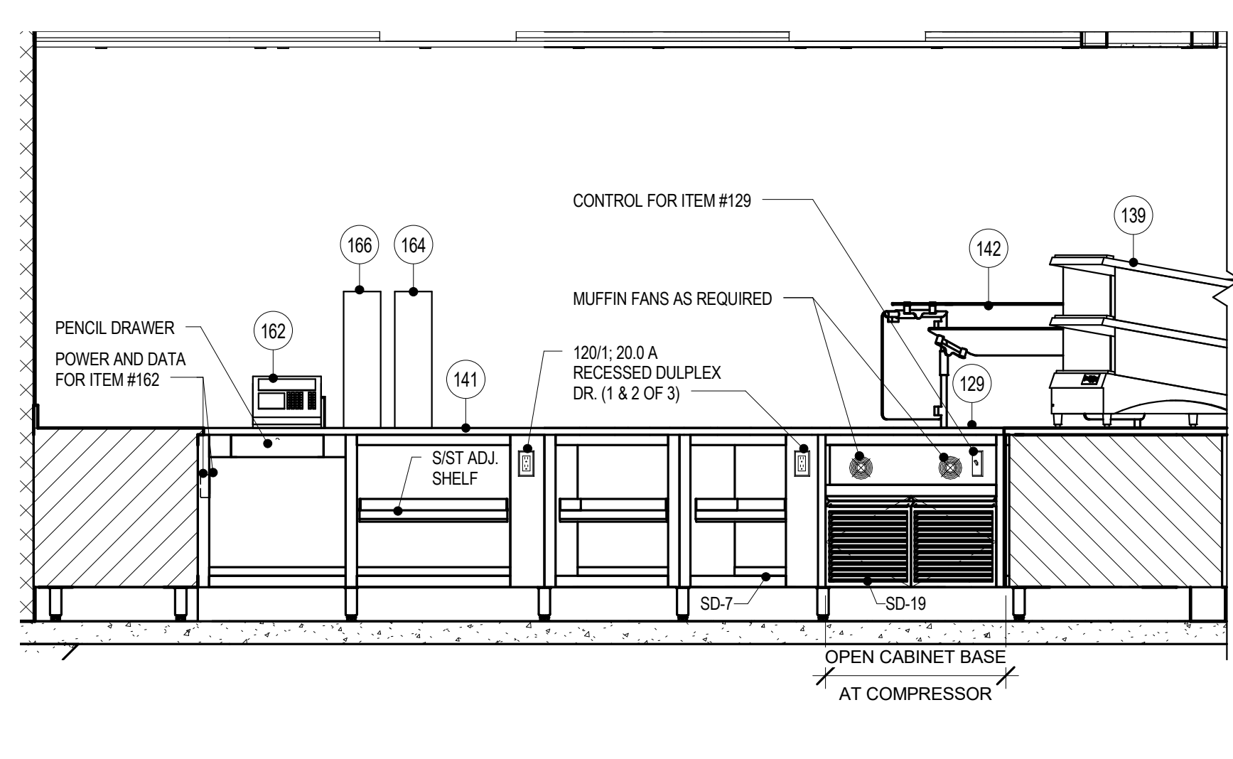
7 ITEM #141 - SERVING COUNTER-BACK B 1/2" = 1'-0"
