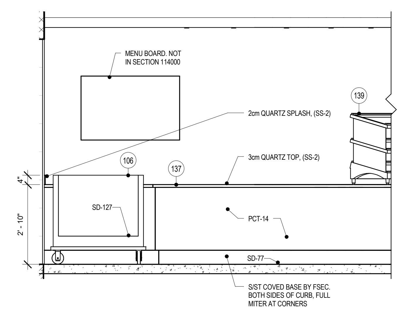
1 ITEM #137 - SERVING COUNTER-FRONT A 1/2" = 1'-0"
