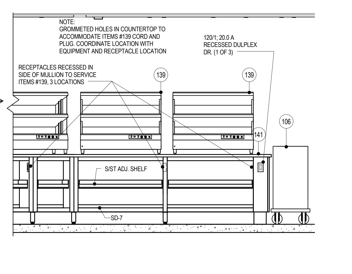
8 ITEM #141 - SERVING COUNTER-BACK A 1/2" = 1'-0"
