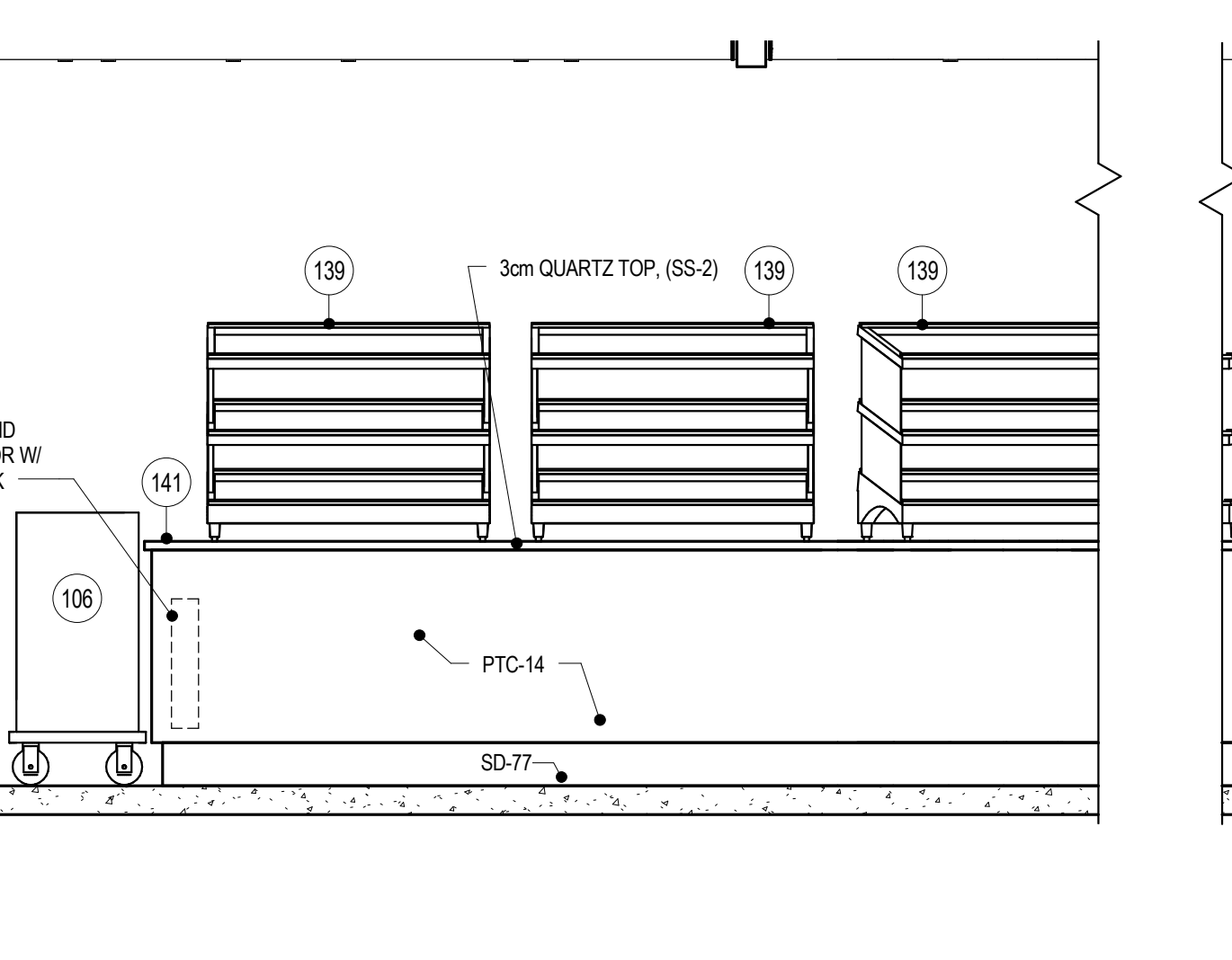
5 ITEM #141 - SERVING COUNTER-FRONT A 1/2" = 1'-0"
