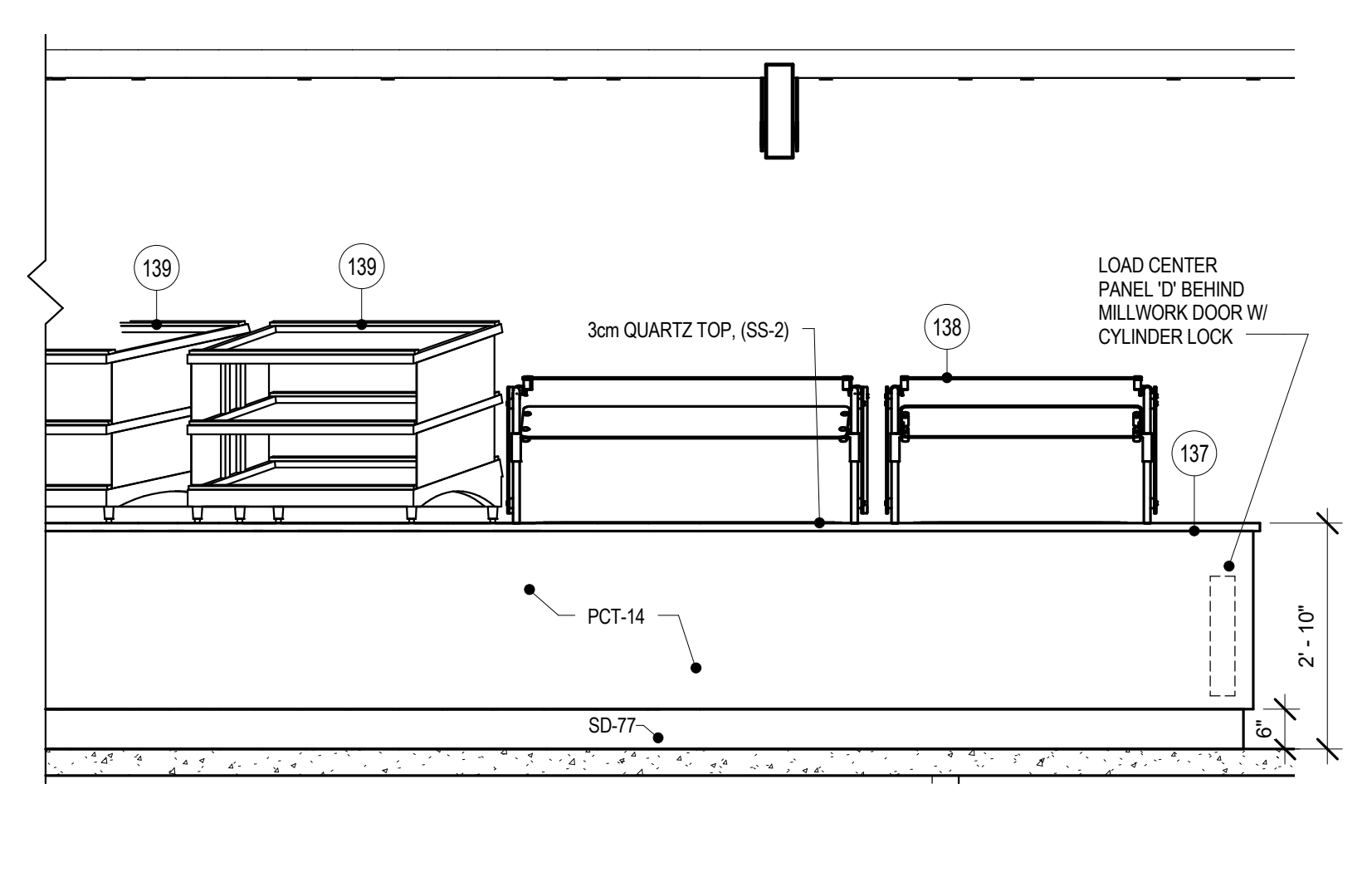
2 ITEM #137 - SERVING COUNTER-FRONT B 1/2" = 1'-0"
