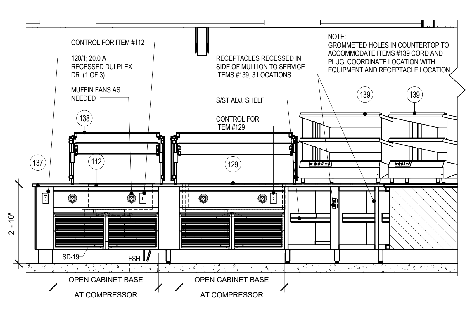
3 ITEM #137 - SERVING COUNTER-BACK A 1/2" = 1'-0"
