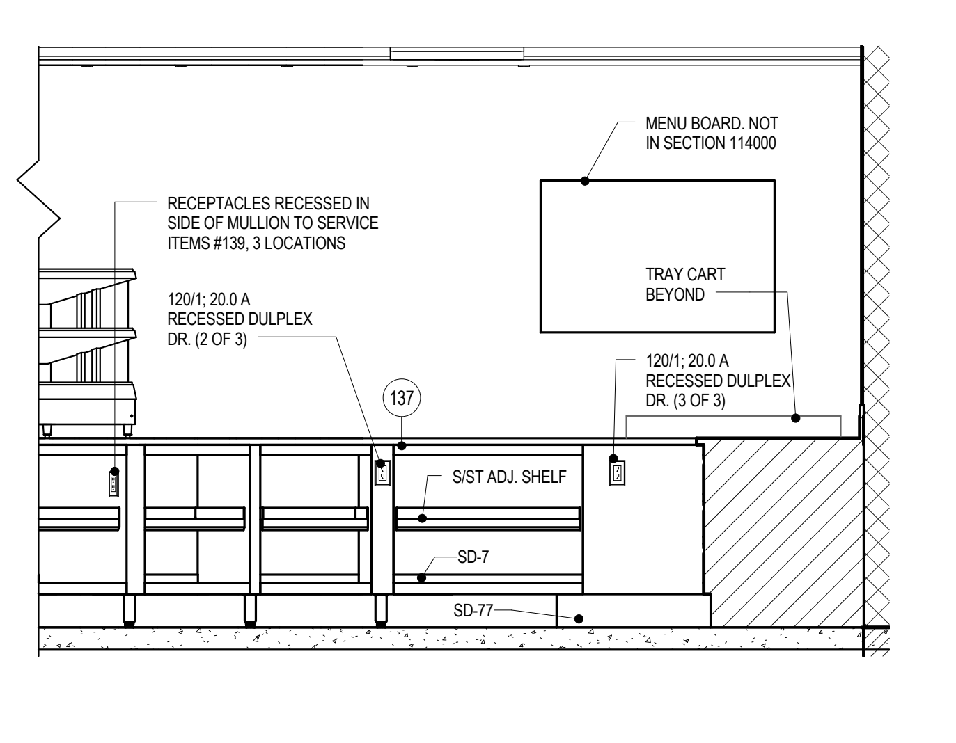
4 ITEM #137 - SERVING COUNTER-BACK B 1/2" = 1'-0"
