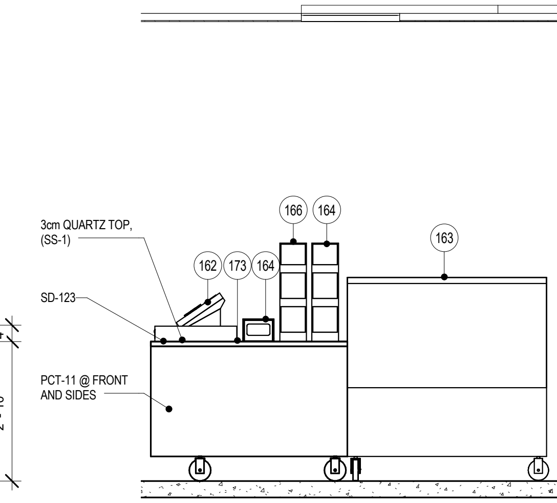
4 ITEM #173 - MOBILE CASHIER STAND 1/2" = 1'-0"
