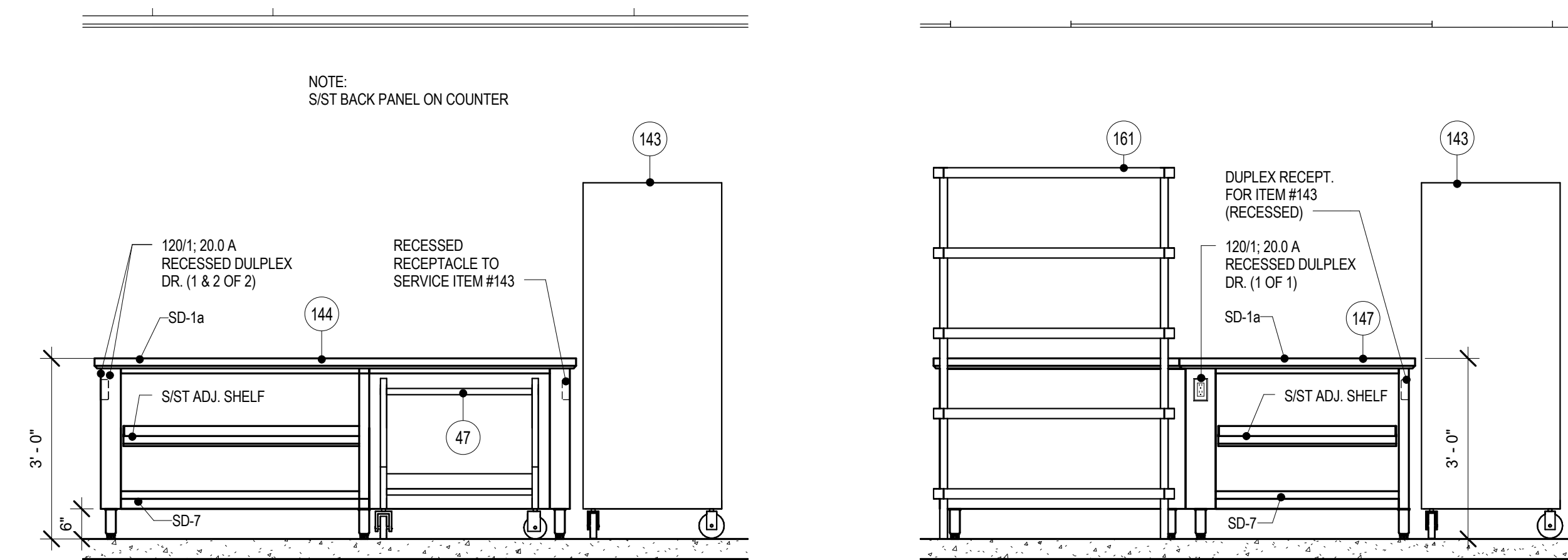
1 ITEM #144 - WORKCOUNTER 1/2" = 1'-0"
