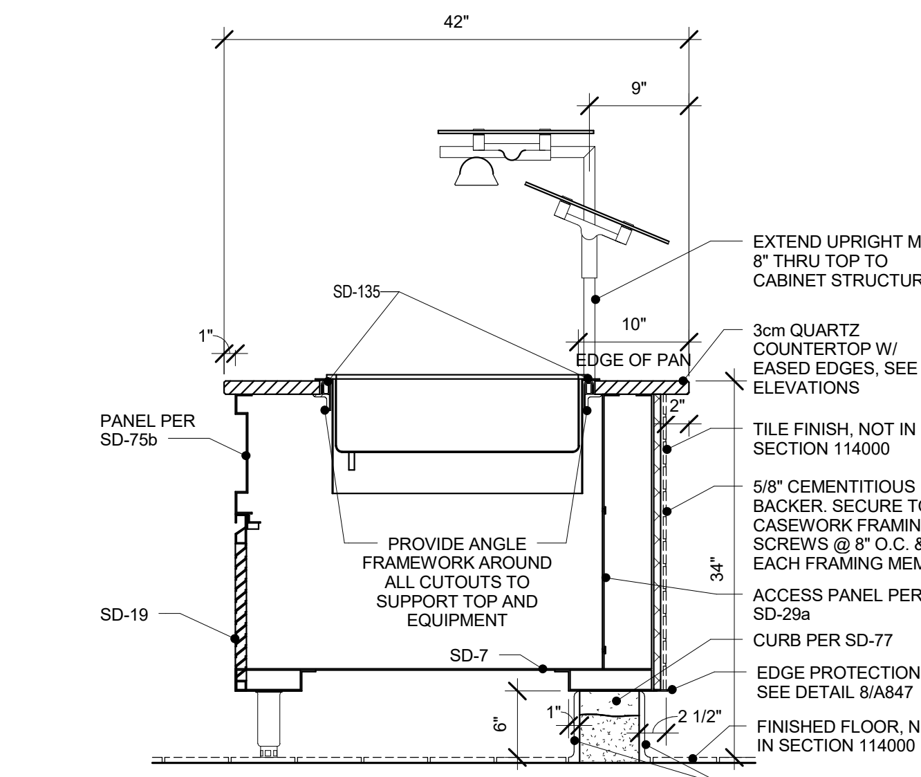
6 SECTION THRU HOT WELL-TILE 1" = 1'-0"
