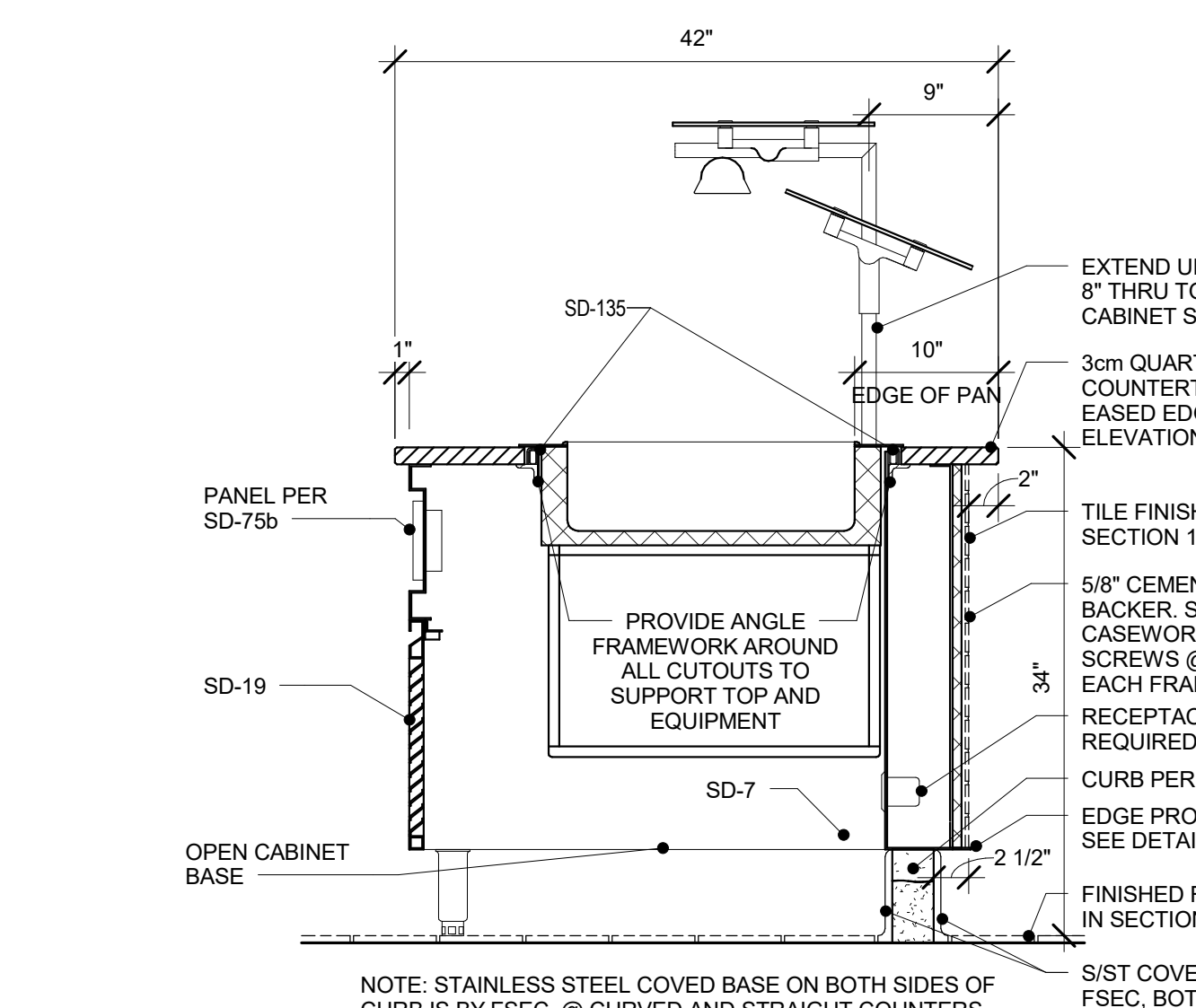
7 SECTION THRU HOT/COLD WELL-TILE 1" = 1'-0"
