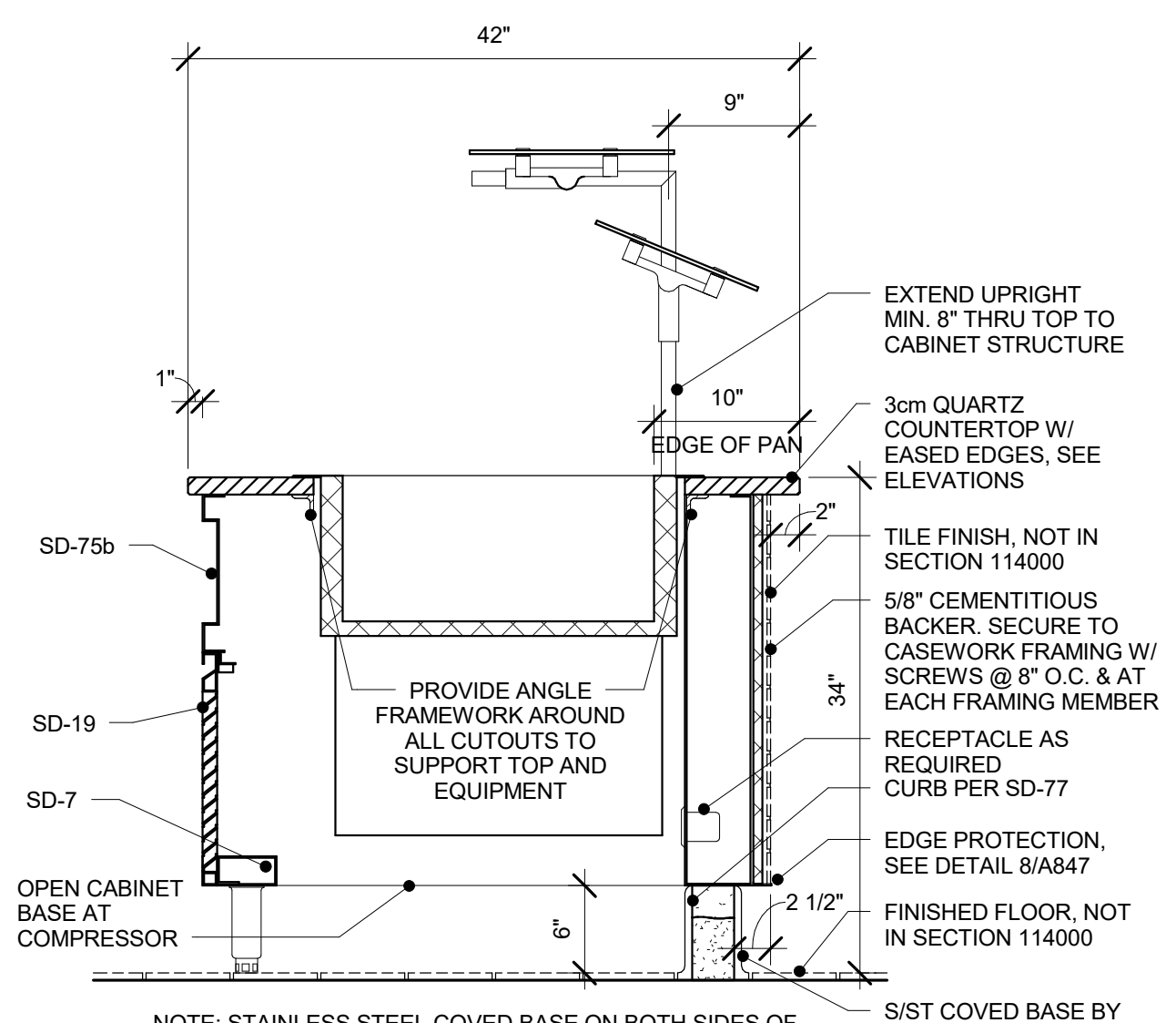
5 SECTION THRU COLD WELL-TILE 1" = 1'-0"
