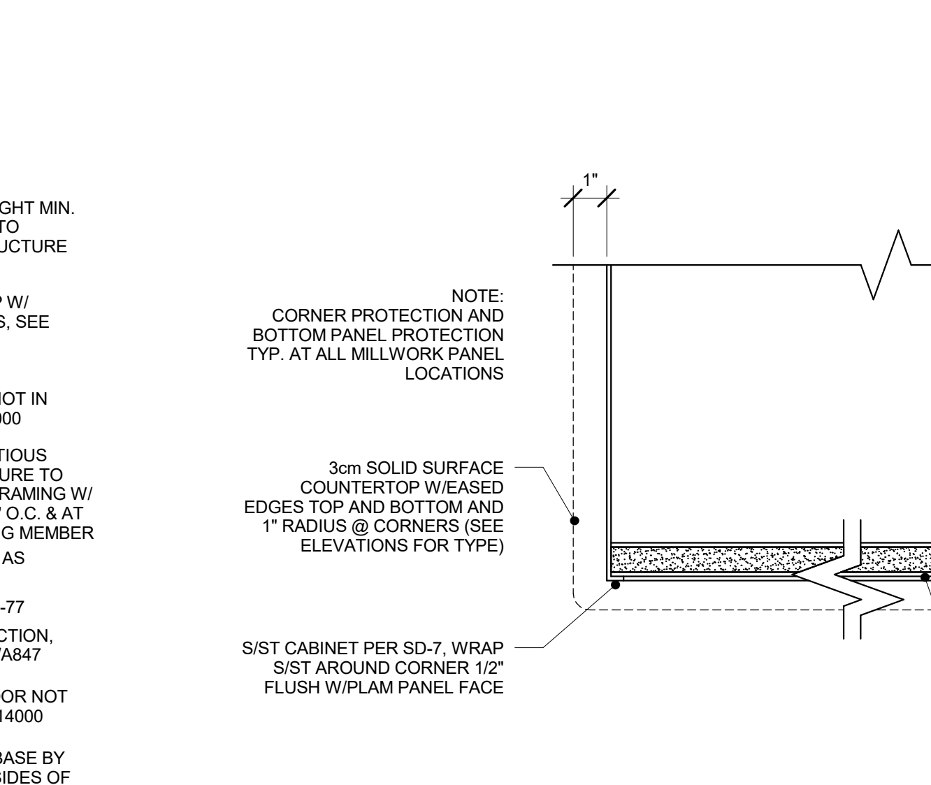
8 TYPICAL EDGE PROTECTION DETAIL 3" = 1'-0"
